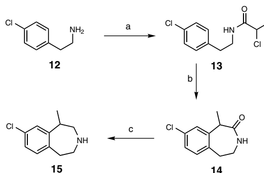
Scheme 2. Reagents and conditions: (a) CH 3 CHClCOCl, pyridine, CH 2 Cl 2 ; (b) AlCl 3 , 150–200 °C; (c) BH 3 , ether.
