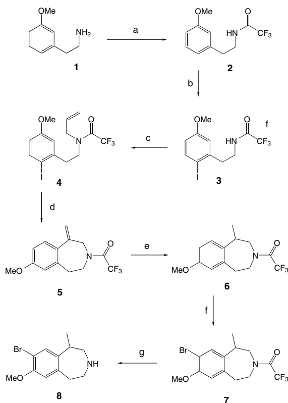
Scheme 1. Reagents and conditions: (a) (CF 3 CO) 2 O, pyridine, CH 2 Cl 2 ; (b) ICl, MeOH; (c) allylbromide, NaOH, K 2 CO 3 , n -Bu 4 NBr, toluene; (d) Pd(OAc) 2 , various conditions; (e) 10% Pd–C, H 2 , MeOH; (f) NBS, CH 3 CN; (g) NaOH, MeOH–H 2 O.
